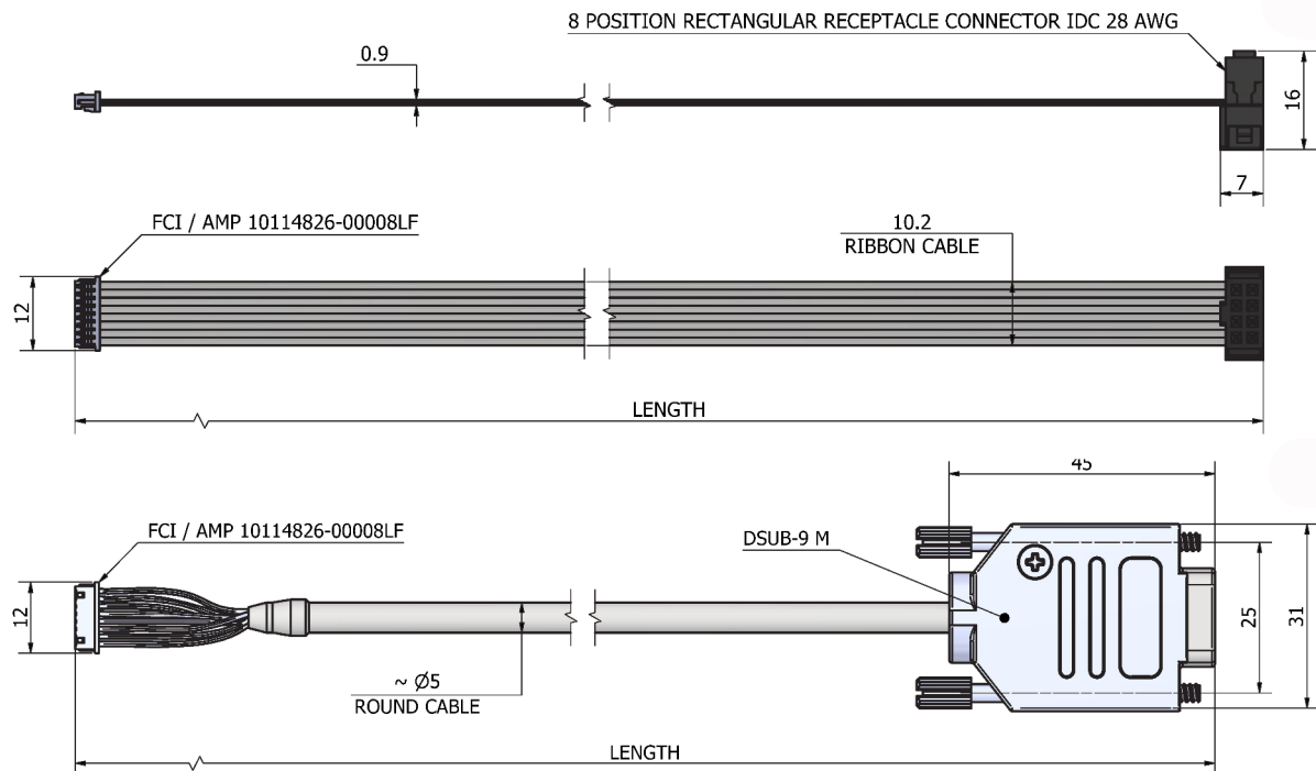
matting connector (AMP 10114826-00008LF)
